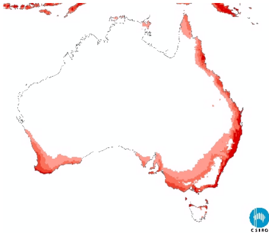
Climate suitability map for myrtle rust (CLIMEX Ecoclimatic Index). Darker red areas indicate higher climate suitability. With microscopic spores that float in the wind there is nothing to stop the spread of myrtle rust in eastern Australia, but its spread to Western Australia may be slowed by quarantine measures, helped by the fact that the prevailing winds typically blow from the west. Credit: Darren Kriticos, CSIRO.
